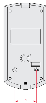
Air2-XDTP200W, Air2-XIRP200W - back
