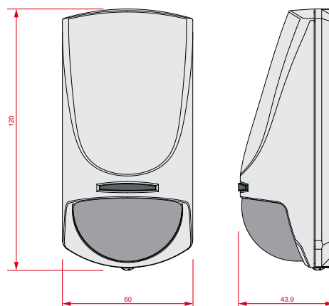
Air2-XDTP200W, Air2-XIRP200W - dimensions
