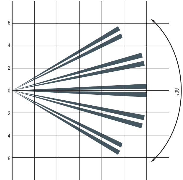
Air2-XIRP200W - top view
