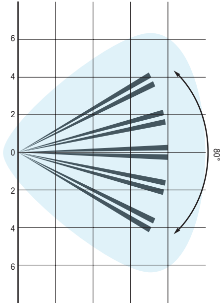
Air2-XIRP200W - top view
