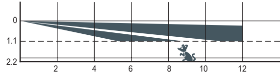
Air2-XIRP200W - side view
