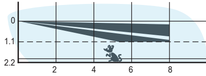
Air2-XDTP200W - side view
